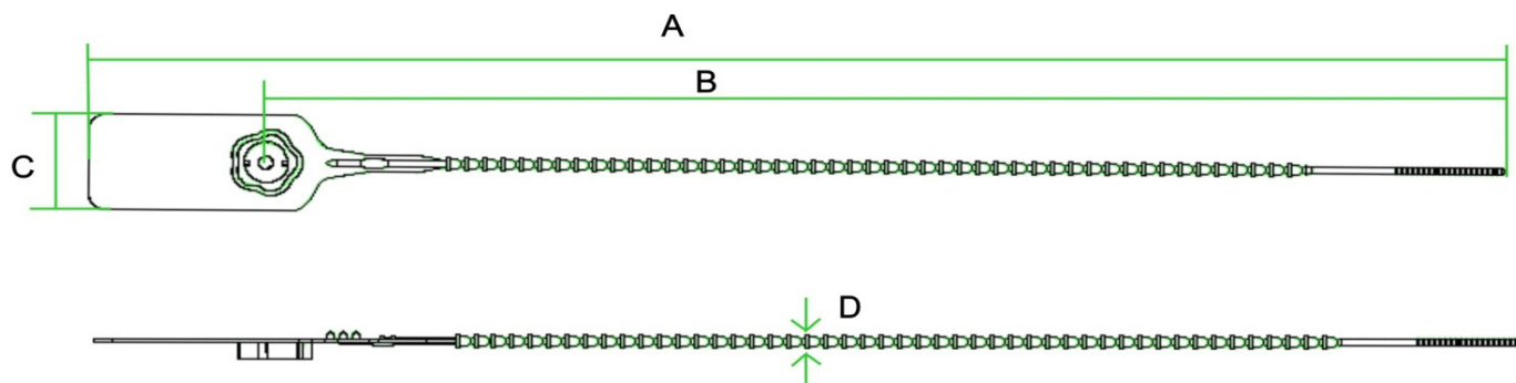
Line Drawing for V-Flex 250mm & 350mm
