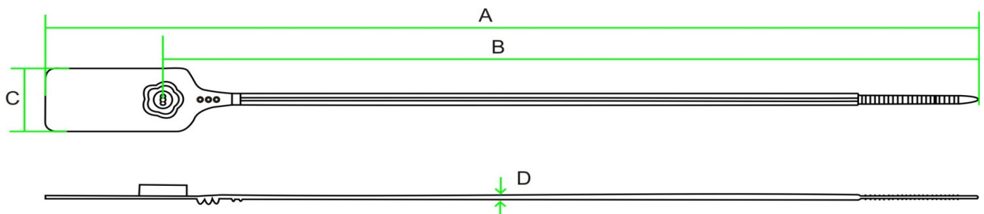
Line Drawing for G-Flex 250mm & 350mm
