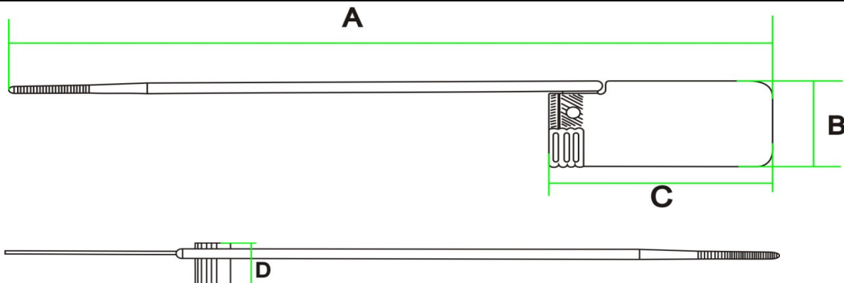
Line Drawing for L-Flex
